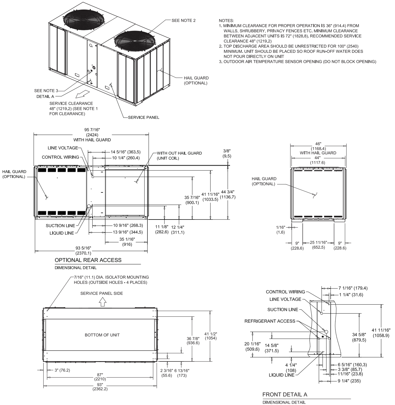
Figure 16. 13-16.7 condensing unit, manifolded compressor, microchannel
