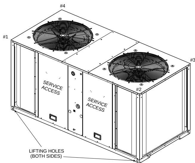
Figure 35. TTA156, 201, 251
