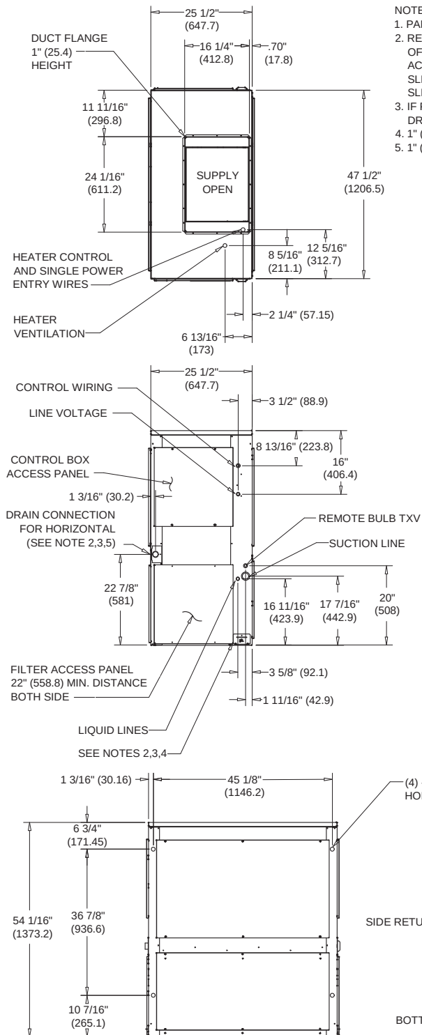
Figure 19. 6, 6.25 ton air handler, single circuit
