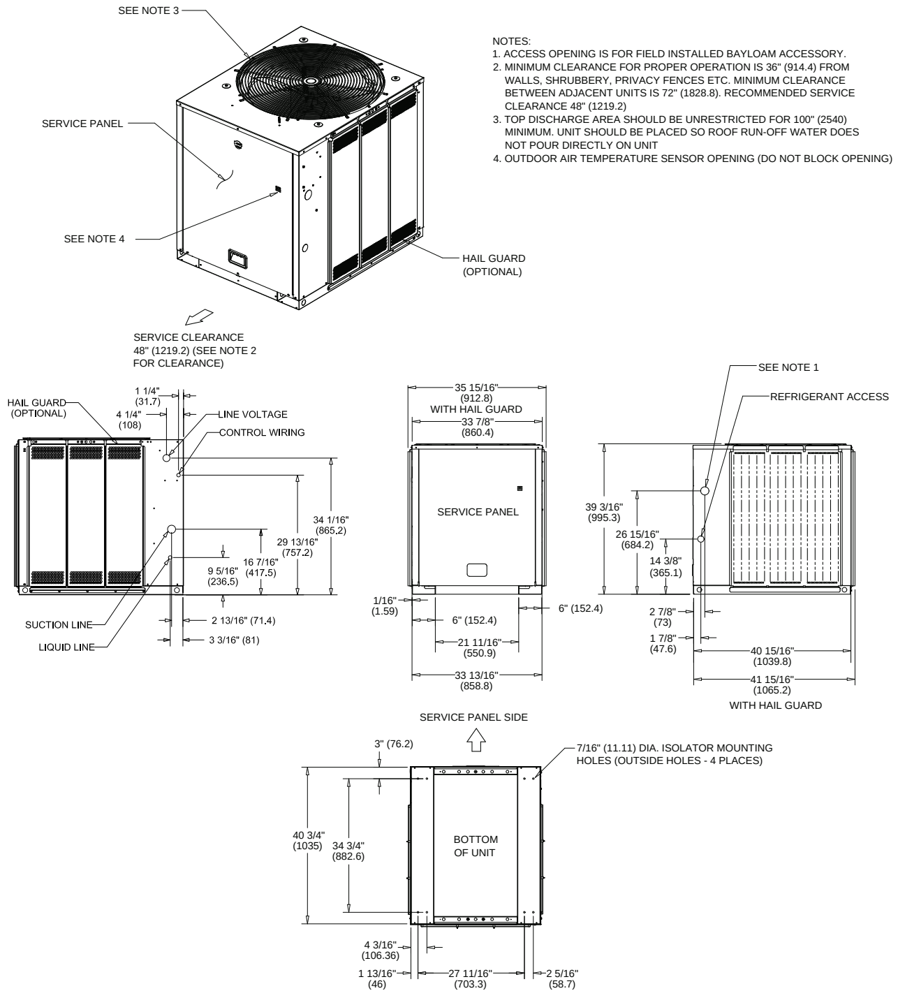
Figure 10. 5-6.25 ton condensing unit, single compressor, microchannel
