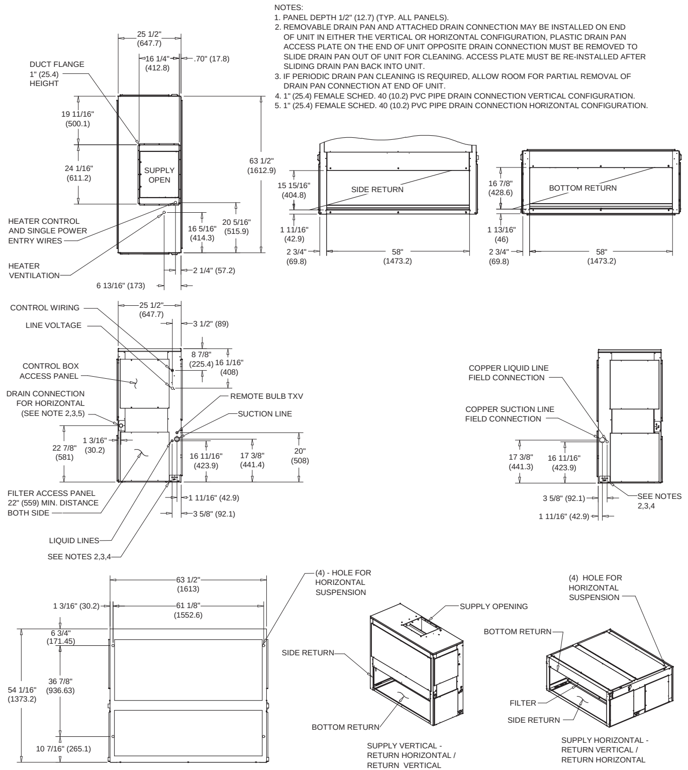
Figure 21. 8.33 ton air handler, single circuit
