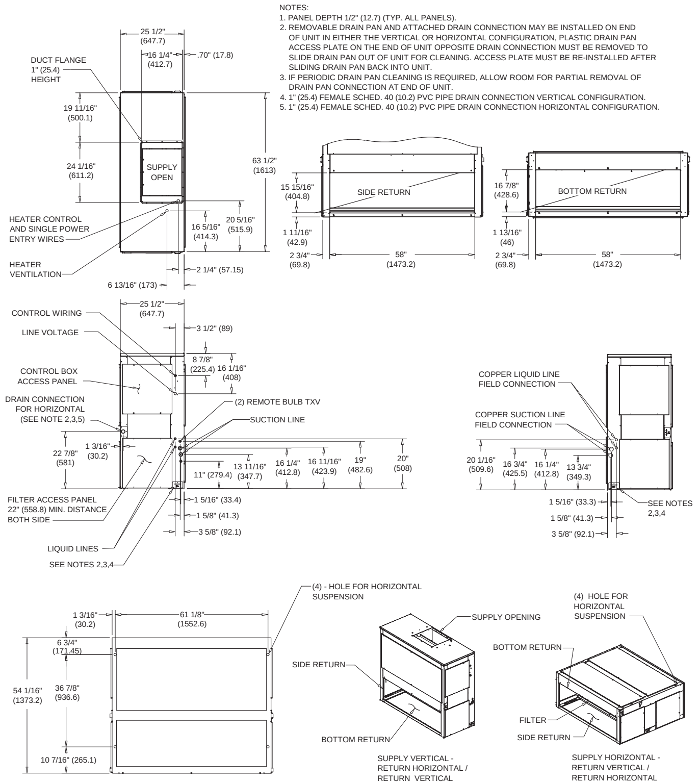
Figure 22. 8.33 ton air handler, dual circuit
