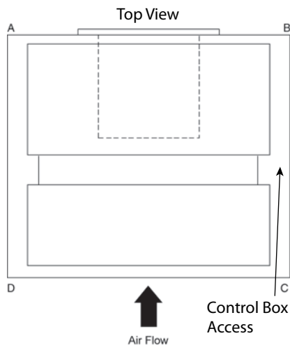
Figure 38. Horizontal — TWE051, 072, 076, 101
