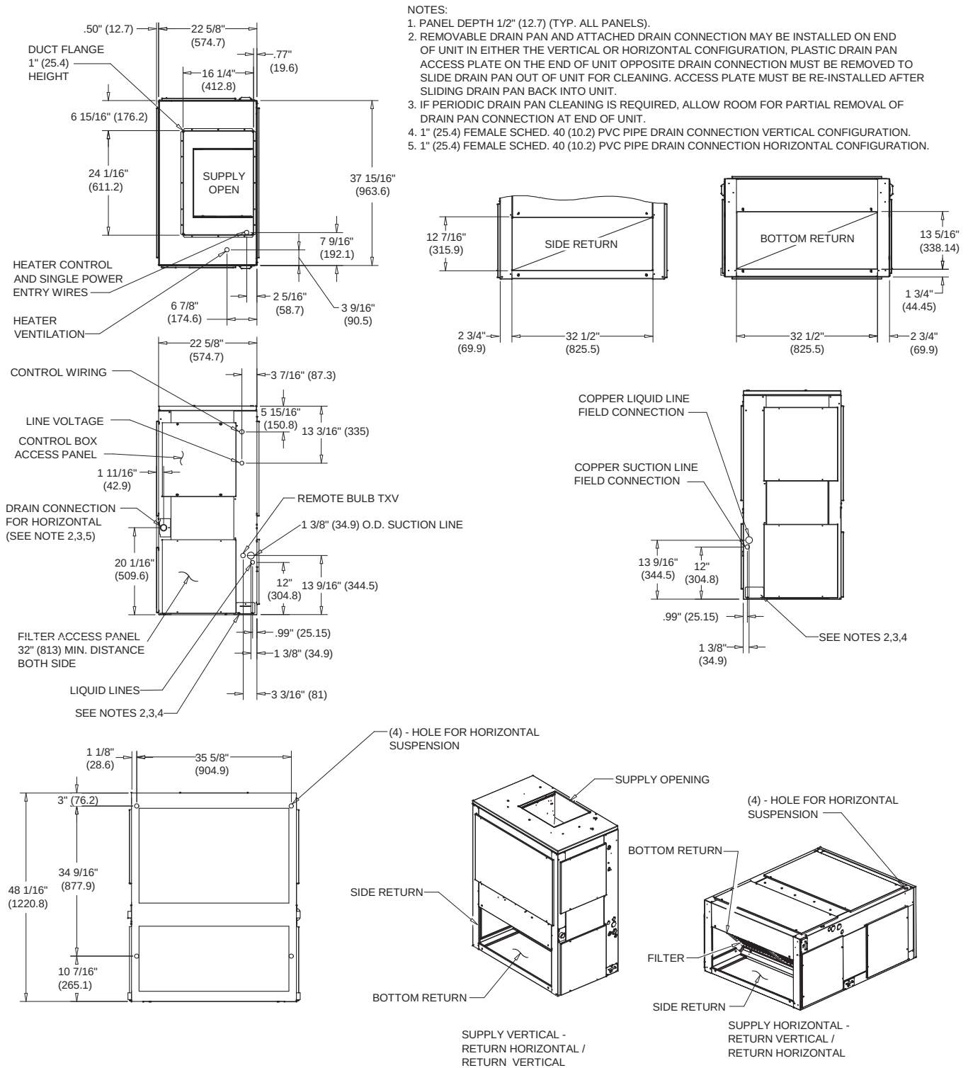
Figure 18. 4.6 ton air handler, single circuit
