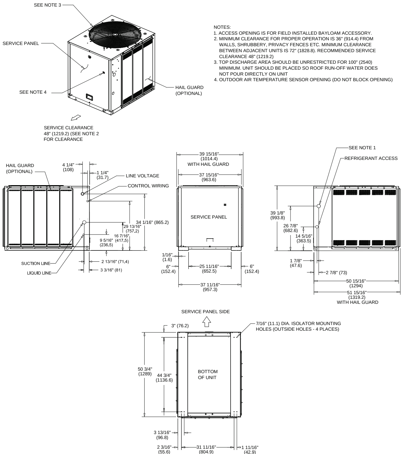
Figure 12. 8.33 ton condensing unit, single and manifolded compressor. microchannel
