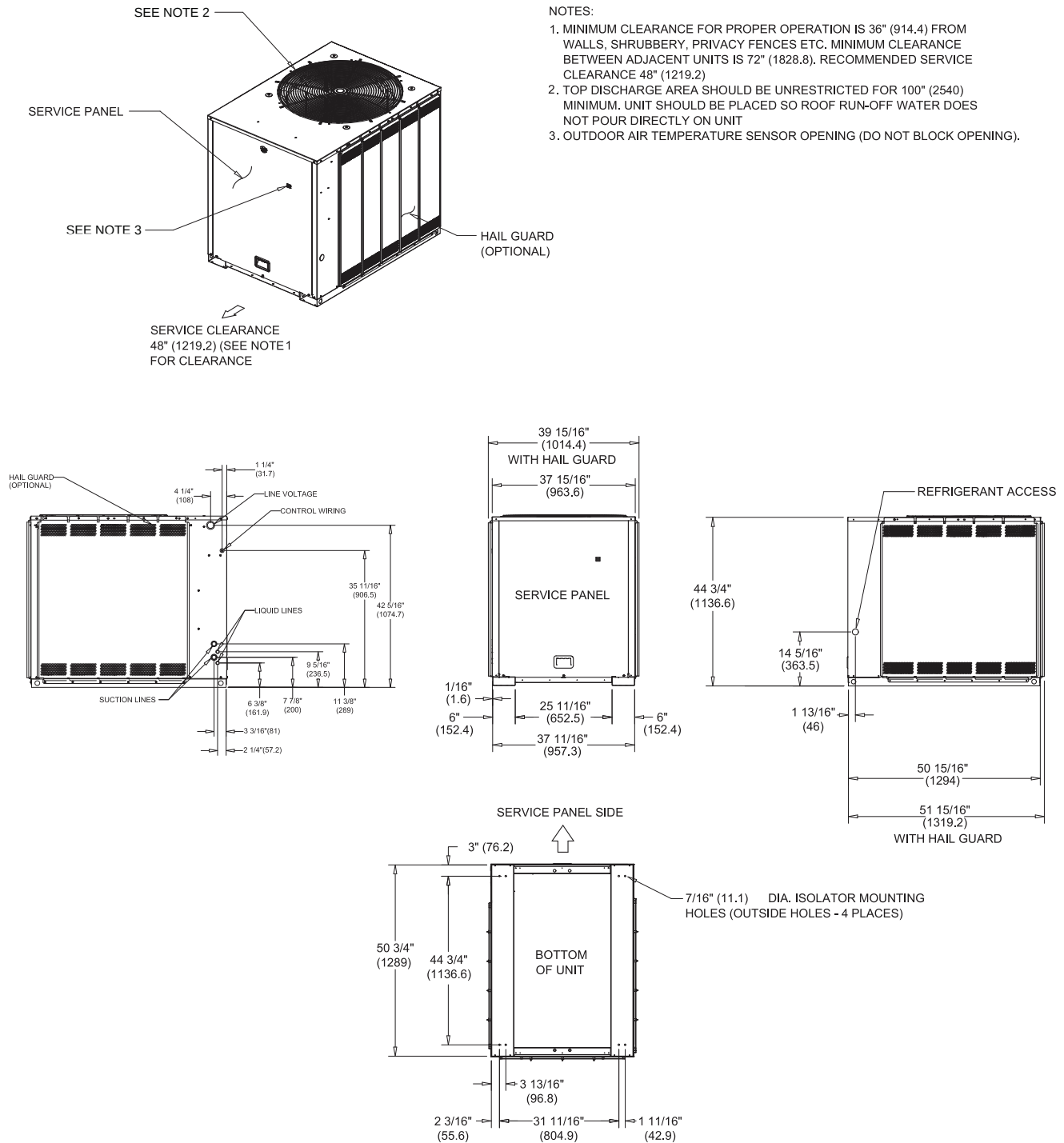
Figure 14. 10.4 ton condensing unit, dual compressor, microchannel
