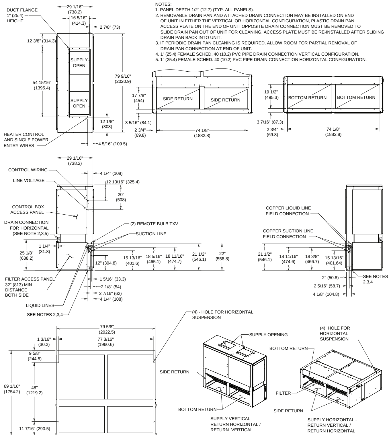
Figure 23. 10.4, 13 ton air handler, dual circuit
