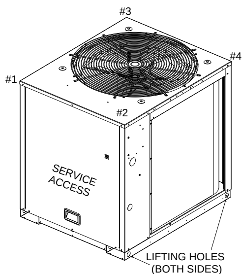
Figure 34. TTA060, 076, 101
