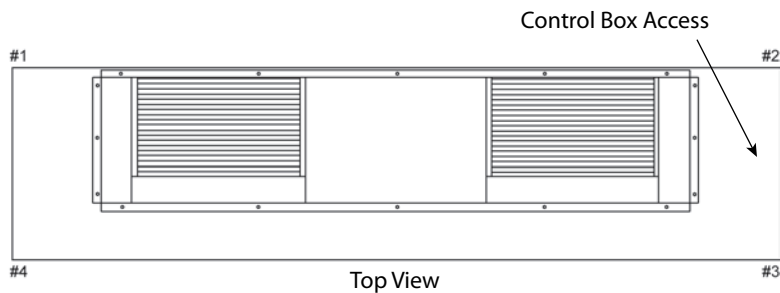
Figure 38. Horizontal — TWE051, 072, 076, 101
