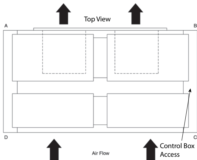
Figure 39. Horizontal — TWE126, 156, 201, 251
