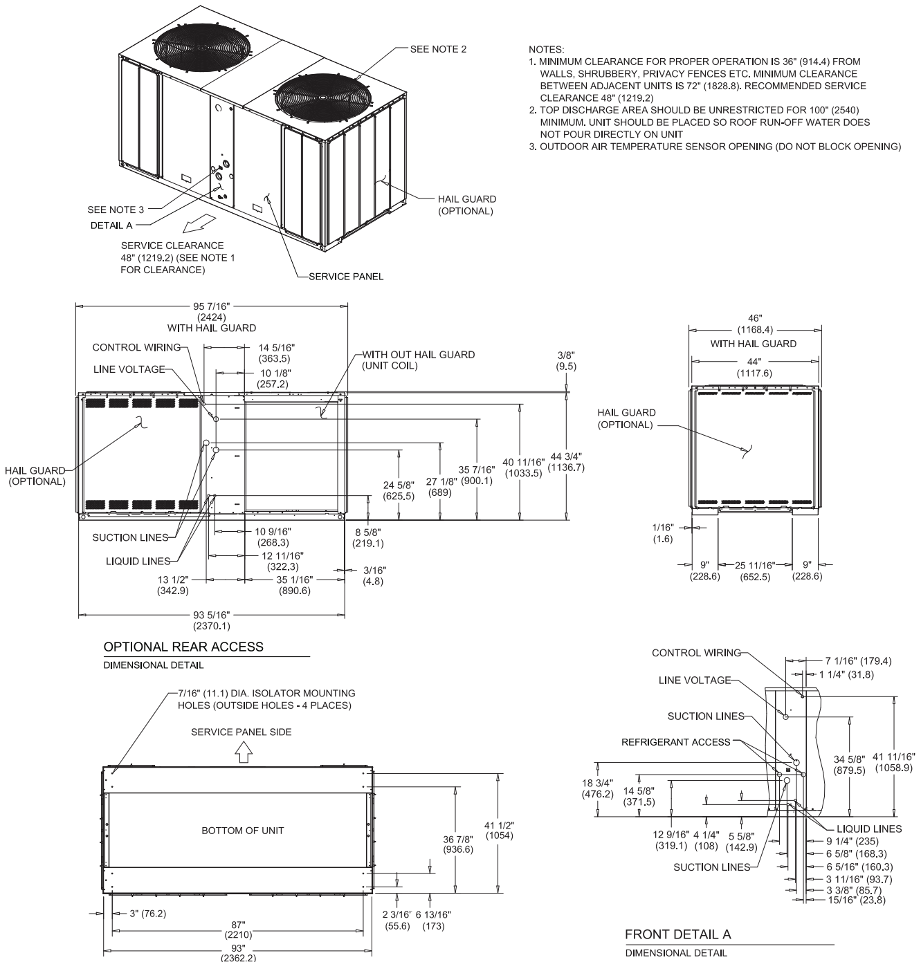
Figure 15. 13-16.7 ton condensing unit, dual compressor, microchannel
